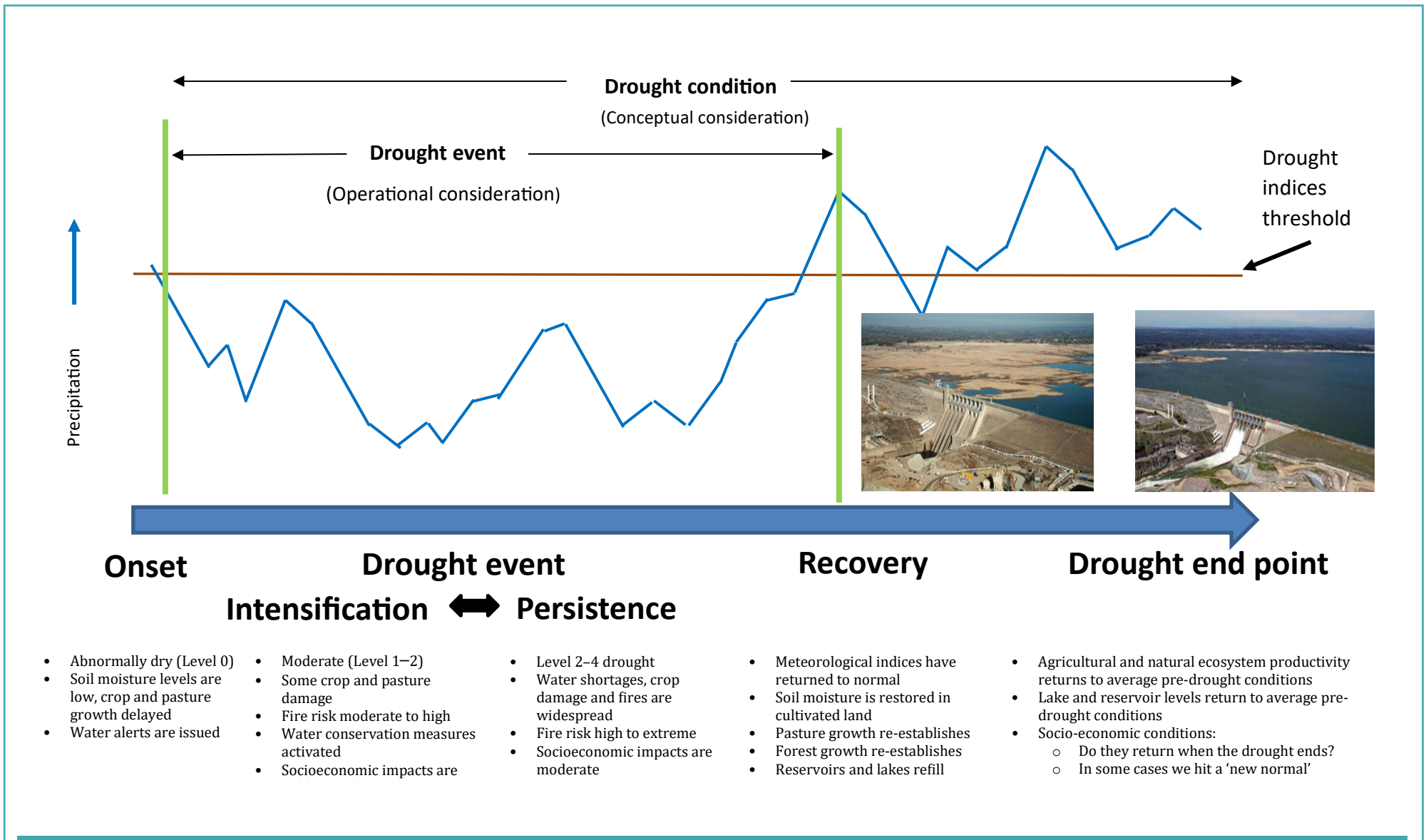
Figure 1.4. Schematic illustration of a drought lifecycle. Source: Howard et al. (in preparation).
