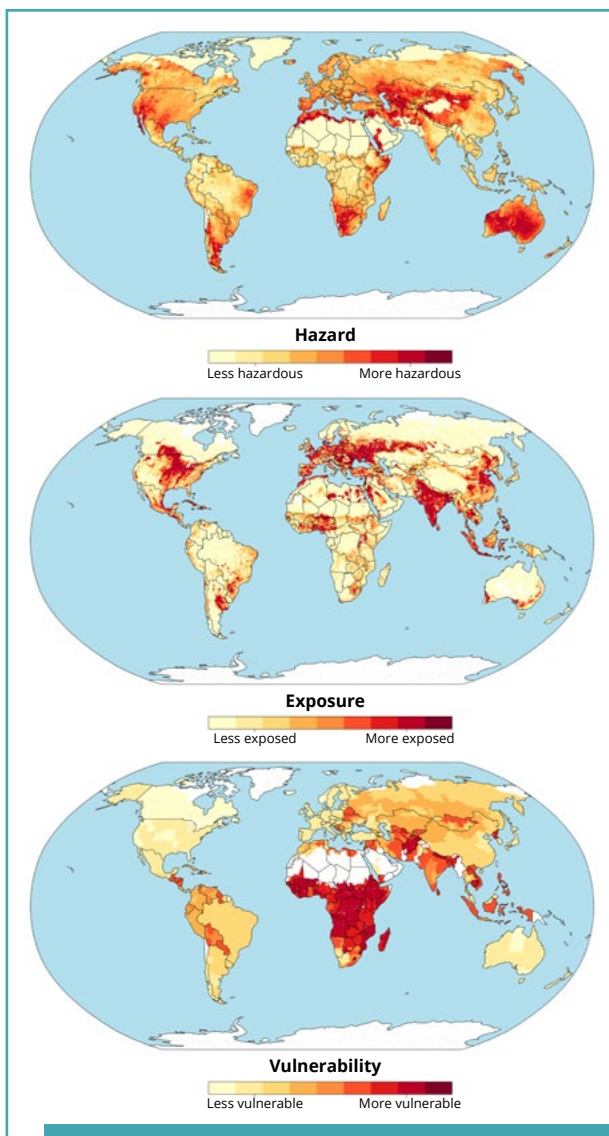
Figure 3.1. Global drought hazard according to the Weighted Anomaly of Standardized Precipitation Index (see also chapter 2), exposure and vulnerability. Source: Vogt et al. (2018).
