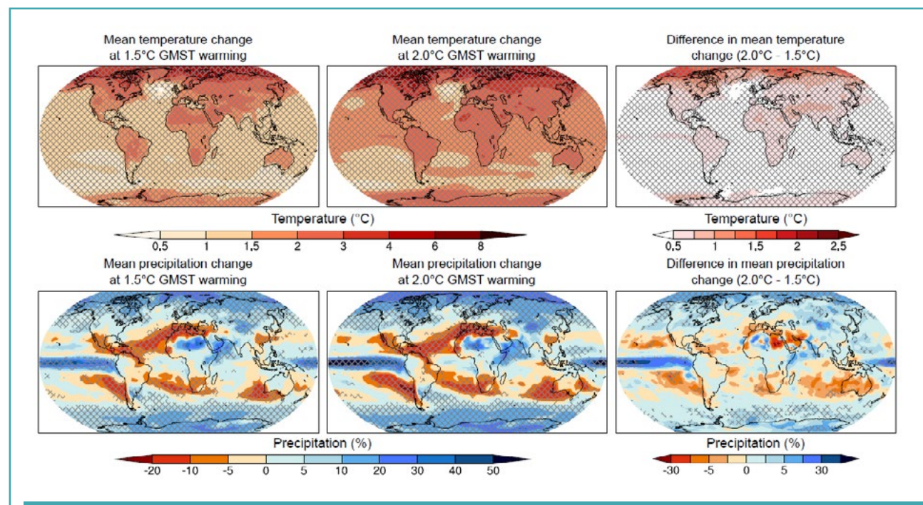
Figure 1.6. Projected changes in mean temperature (top) and mean precipitation (bottom) associated with a rise in surface temperatures of 1.5°C (left) and 2°C (middle), compared to the pre-industrial period (1861–1880), and the difference between the two scenarios (right). Cross-hatching highlights areas where at least two thirds of the models agree on the sign of change as a measure of robustness (18 or more out of 26). Values were assessed from the transient response over a 10-year period at a given warming level, based on Representative Concentration Pathway (RCP) 8.5 Coupled Model Intercomparison Project Phase 5 (CMIP5) model simulations based on Seneviratne et al. (2016) and Wartenburger et al. (2017) (IPCC, 2018). GMST = global mean surface temperatures.
