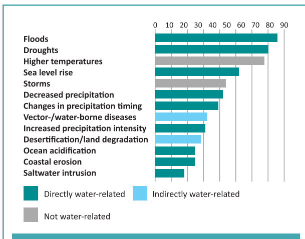
Figure 1.11. Key climate hazards identified in the adaptation components of NDCs. Source: UNFCCC (2016).
